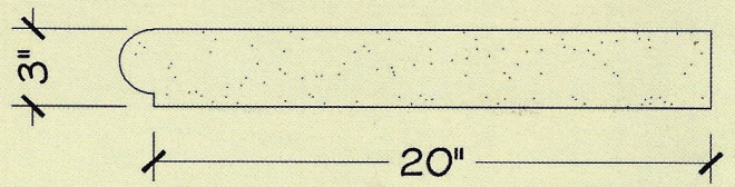
2" BULLNOSE
