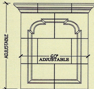
MODEL # - OM600
