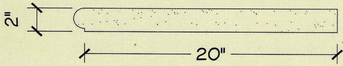
2" BULLNOSE
