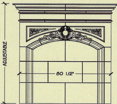
MODEL # - OM500
